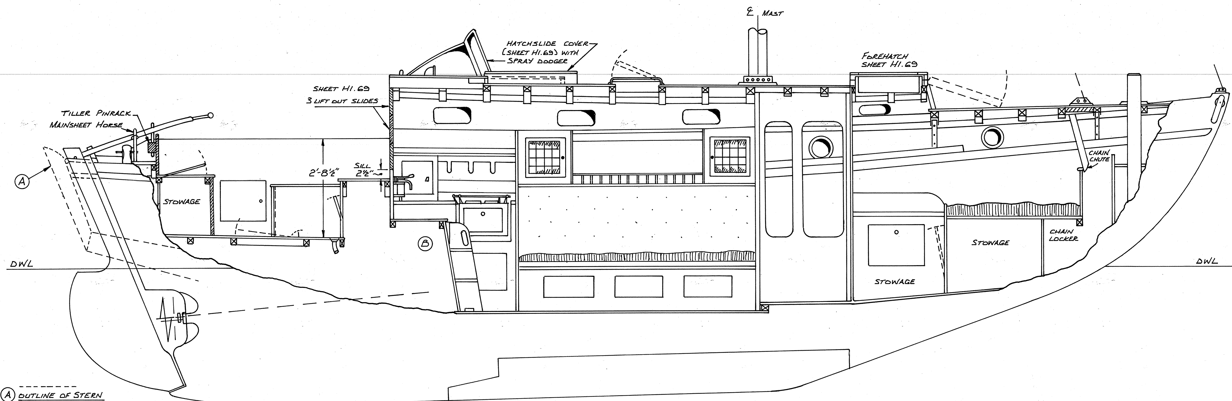
(A) OUTLINE OF STERN FOR NOONTIDE 32 (STEEL-BUILT VERSION)
