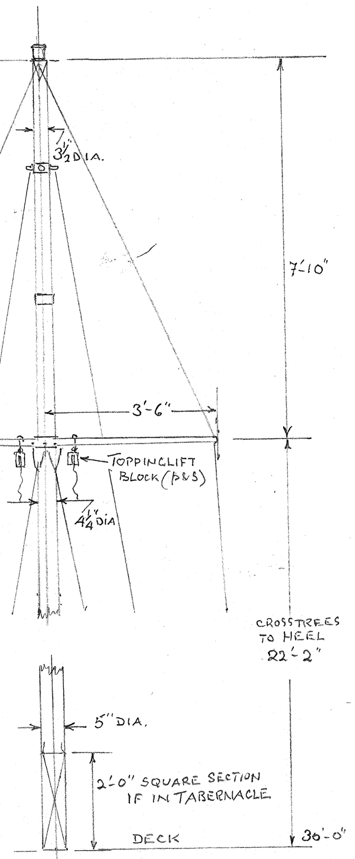
MEASUREMENTS FOR SOLID SPRUCE MAST or similar
