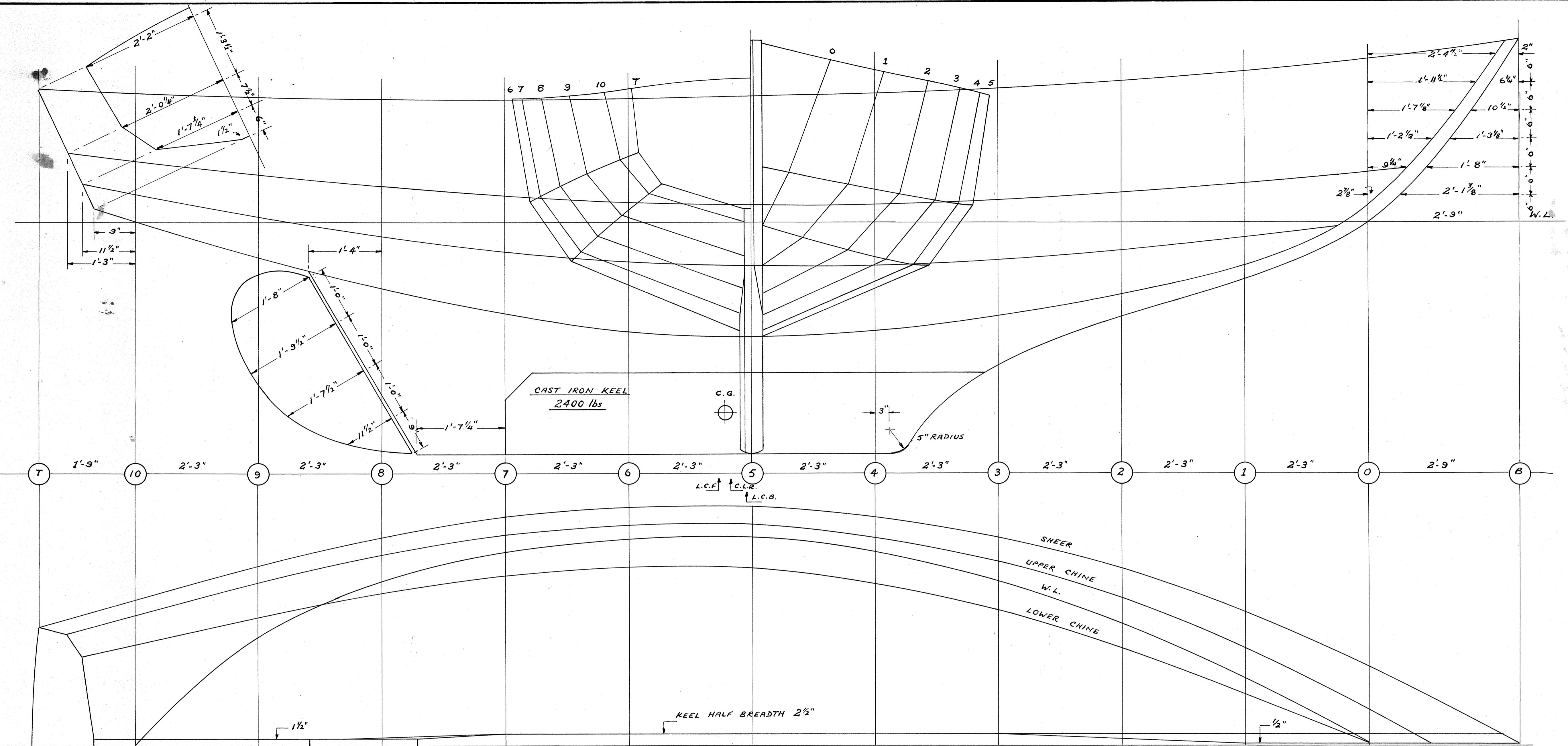
OFFSETS IN FEET, INCHES AND EIGHTHS
