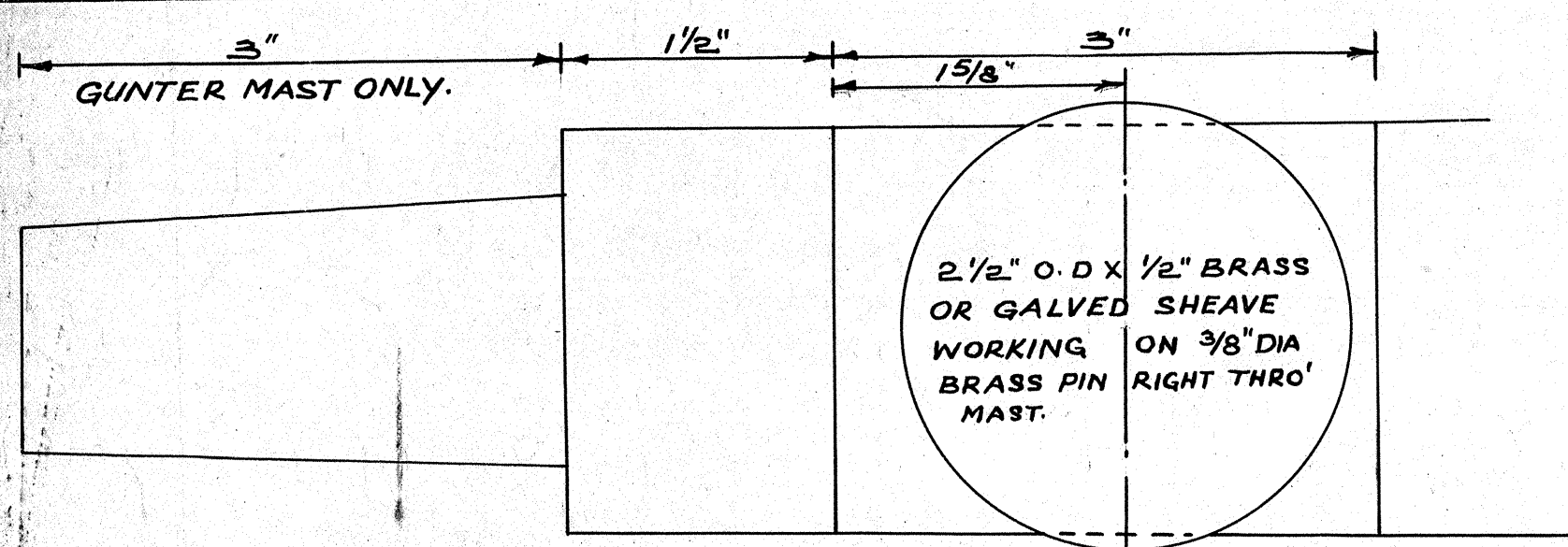
DETAIL OF MASTHEADS.
