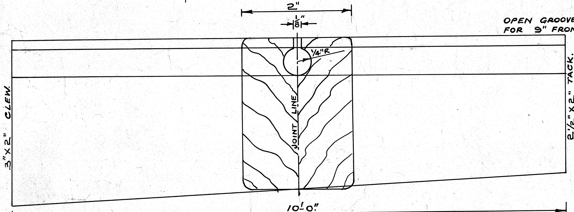
BOOM FOR GUNTER & BERMUDIAN RIG. SILVER SPRUCE. SOLID. MAKE UP IN TWO HALVES WITH FOOT ROPE GROOVE.
