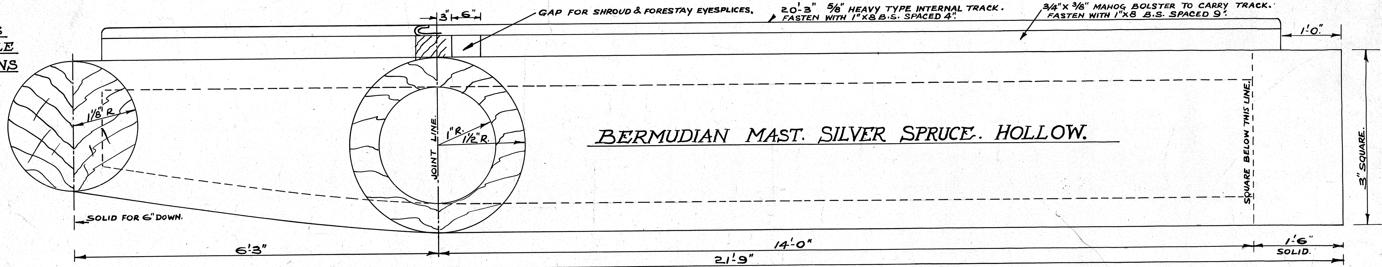
DETAIL OF MASTHEADS.
