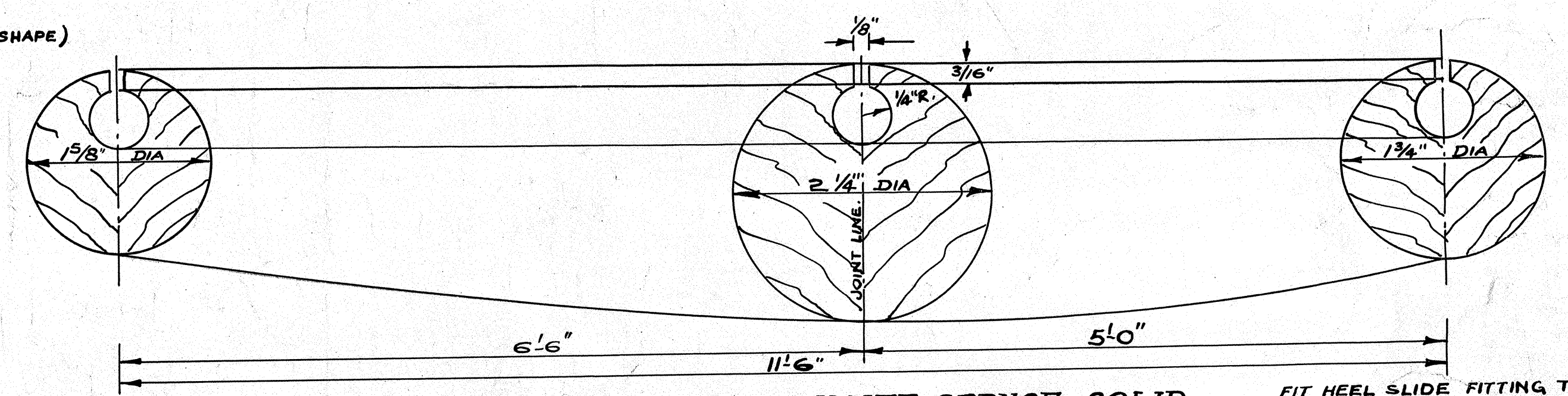
YARD FOR GUNTER RIG. SILVER SPRUCE. SOLID. MAKE UP IN TWO HALVES WITH HEAD ROPE GROOVE.
