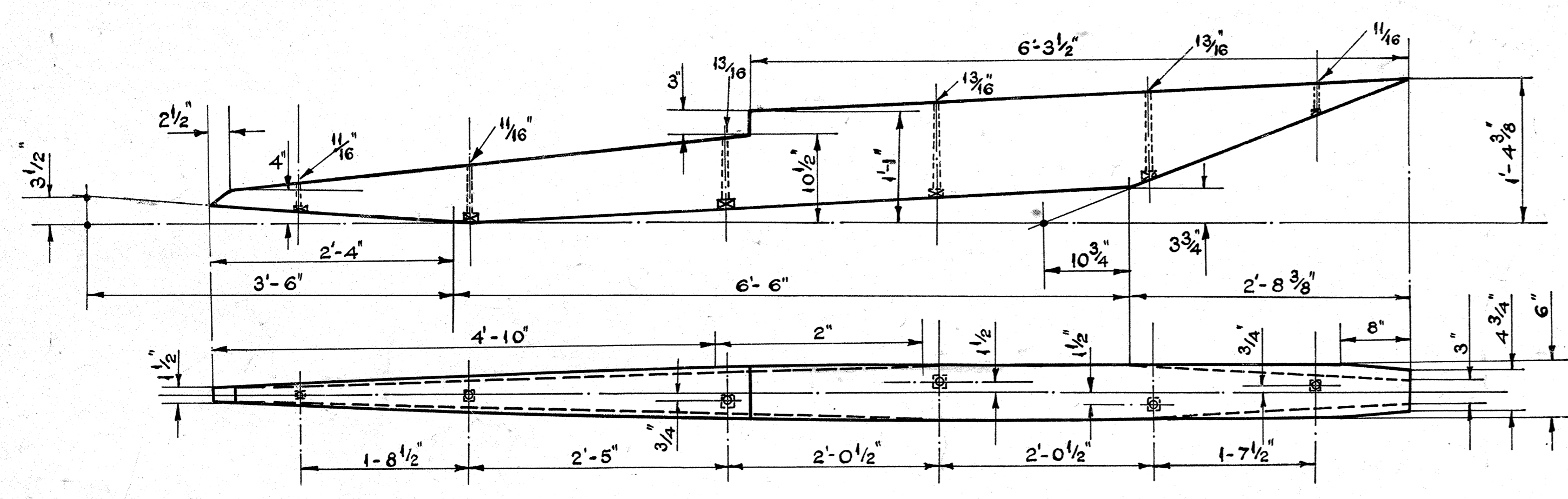
DETAIL OF IRON KEEL. CAST IRON 12 CWT.
