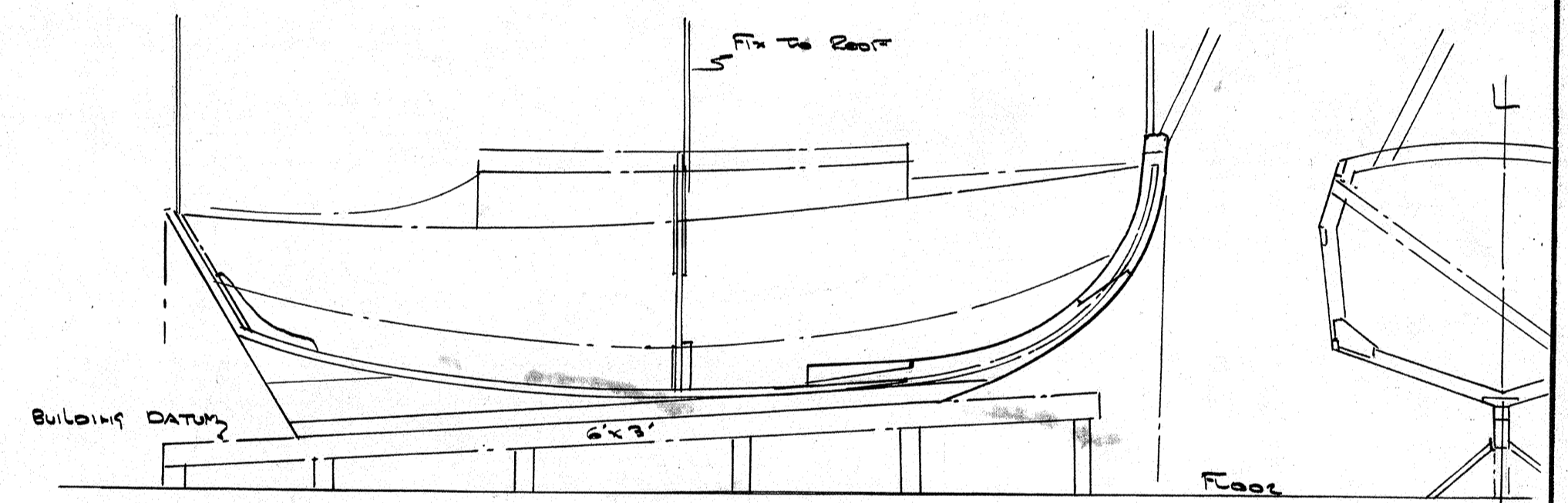
DIAGRAM OF BUILDING SET UP
